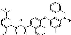
1-(5-tert-Butyl-2-methoxy-phenyl)-3-(4-{6-methyl-2-[(pyridin-2-ylmethyl)-amino]-pyrimidin-4-yloxy}-naphthalen-1-yl)-urea;
